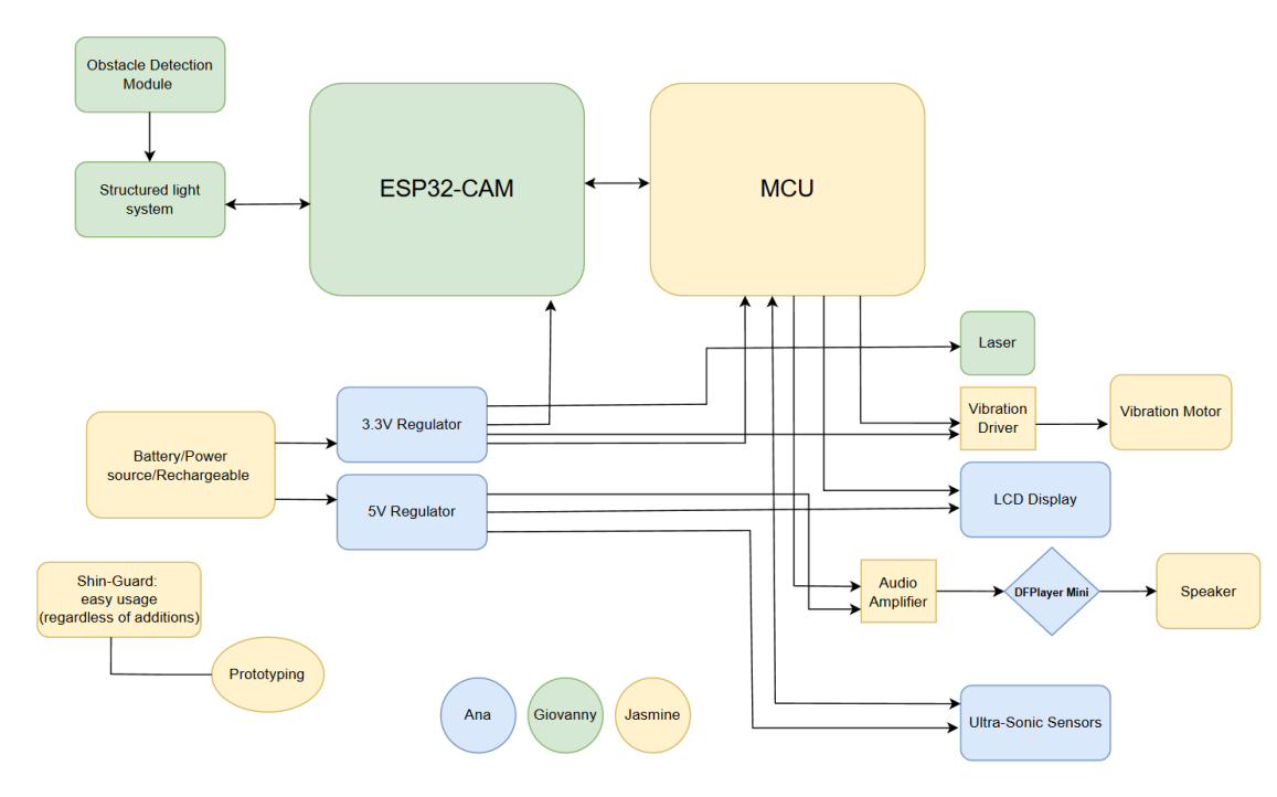
Figure 24: Block Diagram
