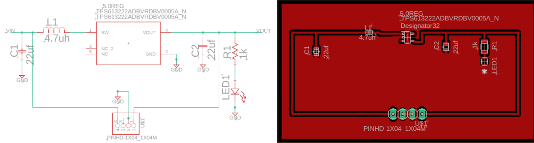
Figure 42: 5.0 Regulator
