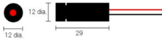
Figure 28: Laser Diagram
