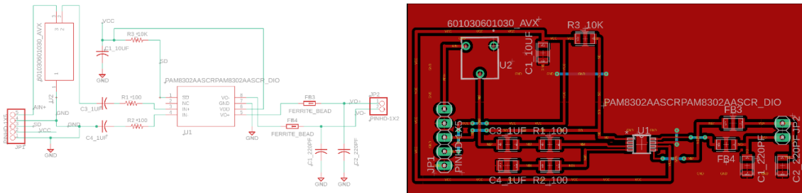
Figure 43: Audio Amplifier
